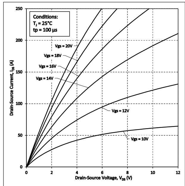
Figure 2. Output Characteristics T_j = 25\text{ }^\circ\text{C}
