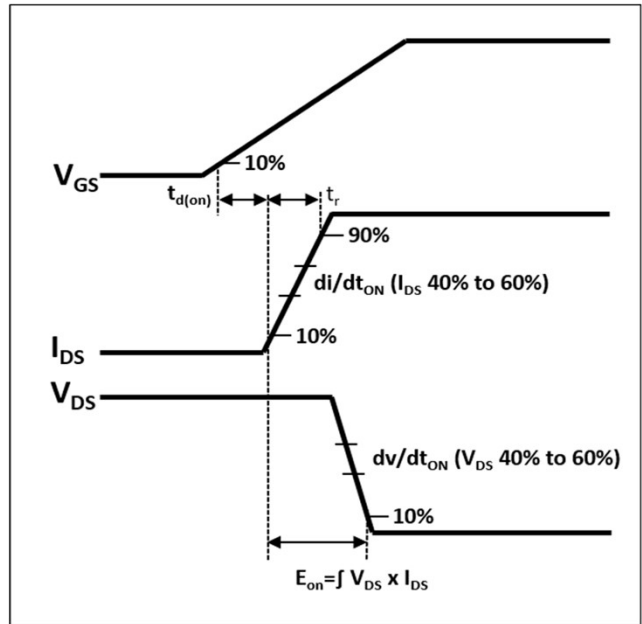
Figure 32. Turn-on Transient Definitions
