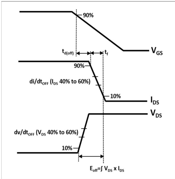
Figure 31. Turn-off Transient Definitions
