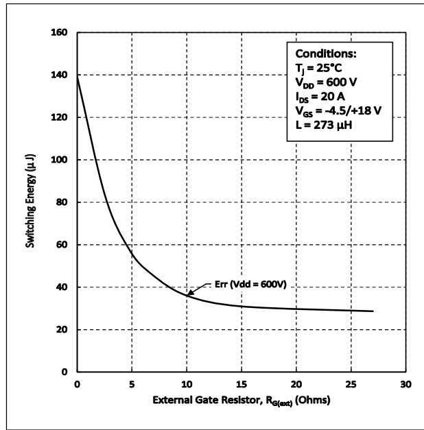
Figure 24. Reverse Recovery Energy vs. R_{G(\text{ext})}
