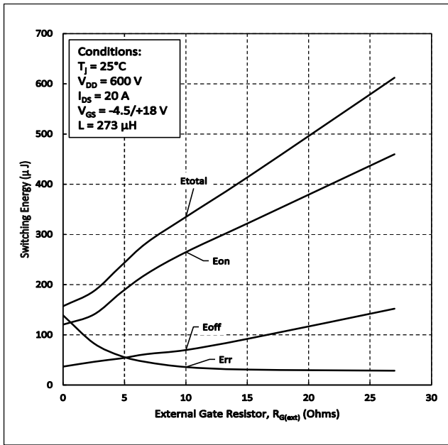
Figure 23. Clamped Inductive Switching Energy vs. R_{G(\text{ext})}
