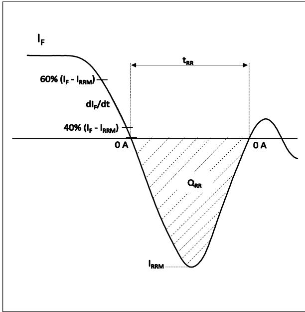
Figure 33. Reverse Recovery Definitions
