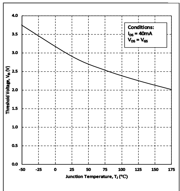
Figure 12. Threshold Voltage vs. Temperature
