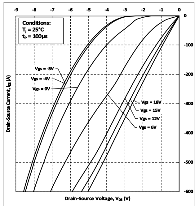
Figure 10. Body Diode Characteristics at T_j = 25^\circ\text{C}
